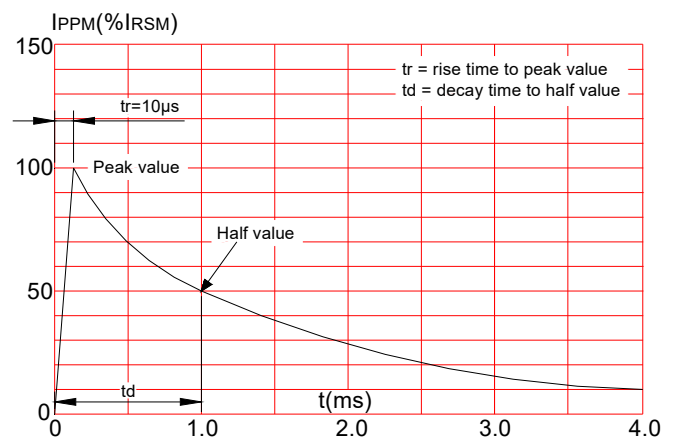
FIG.4: Pulse waveform
