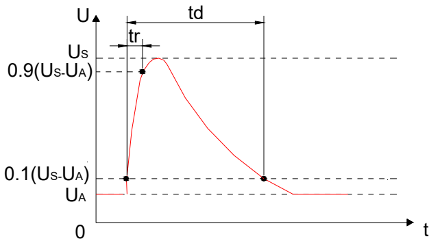
FIG.7: ISO16750 -2 test pulse 5a
