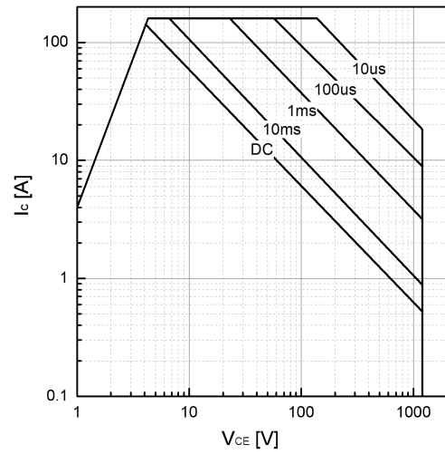
Fig 14. Safe operating area
